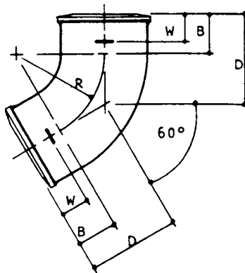
FIG. 15 7 1/2° Bend (corresponds to Table 19 of CISPI Specification 301)
